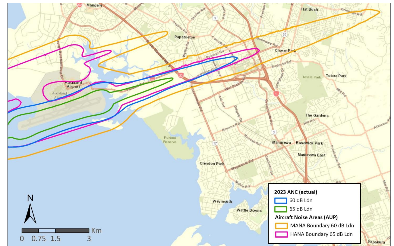
Figure 5: 2023 Actual Noise Contour (ANC)
